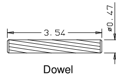
Dowel
