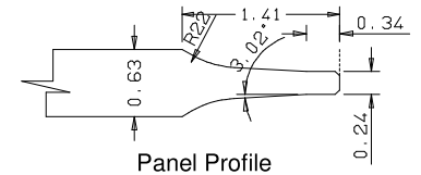
Panel Profile
