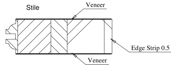
Panel Profile
