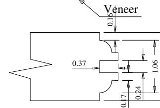
Profile
