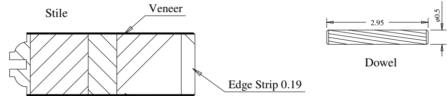
Panel Profile
